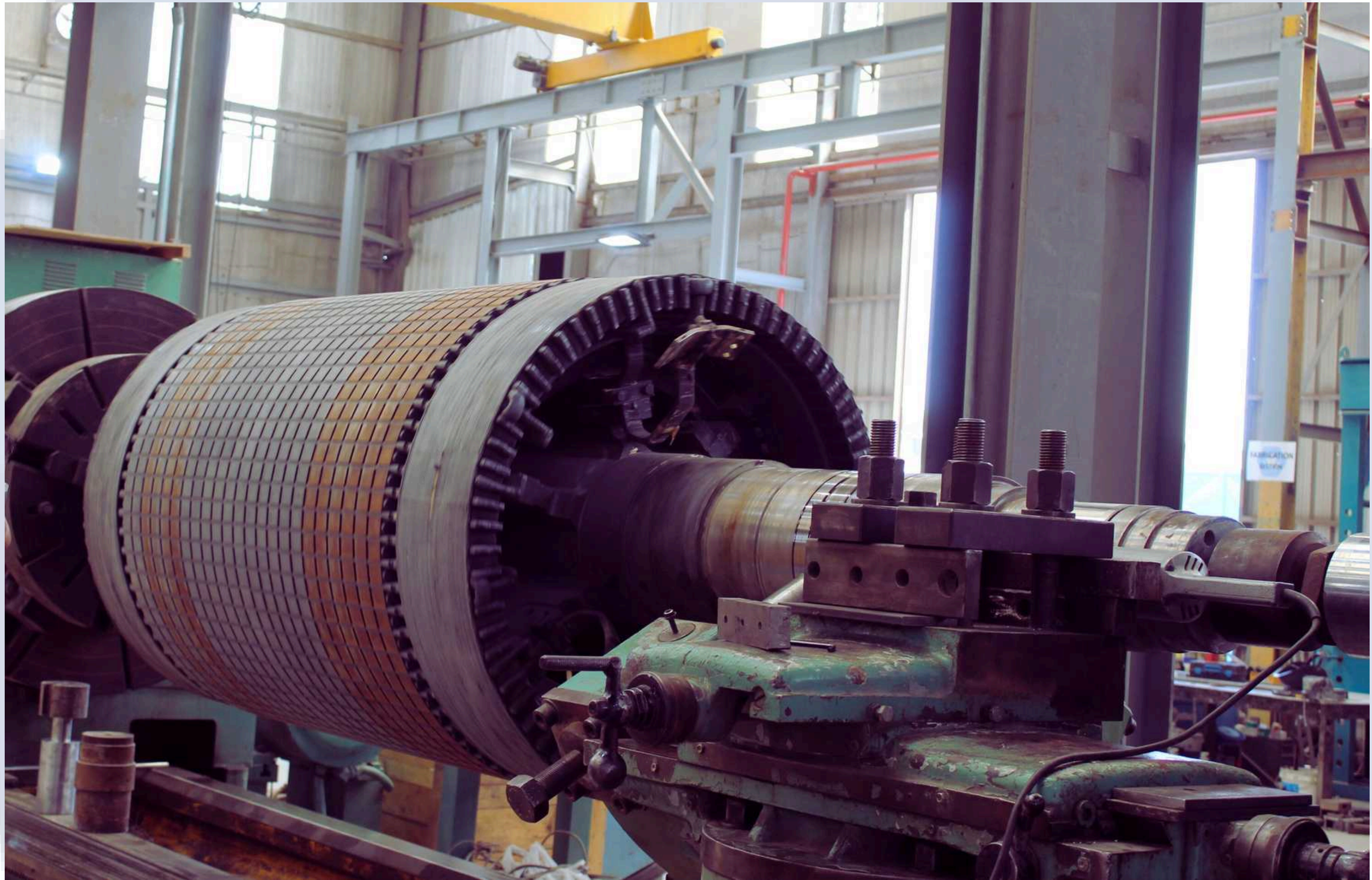
Machining Section
