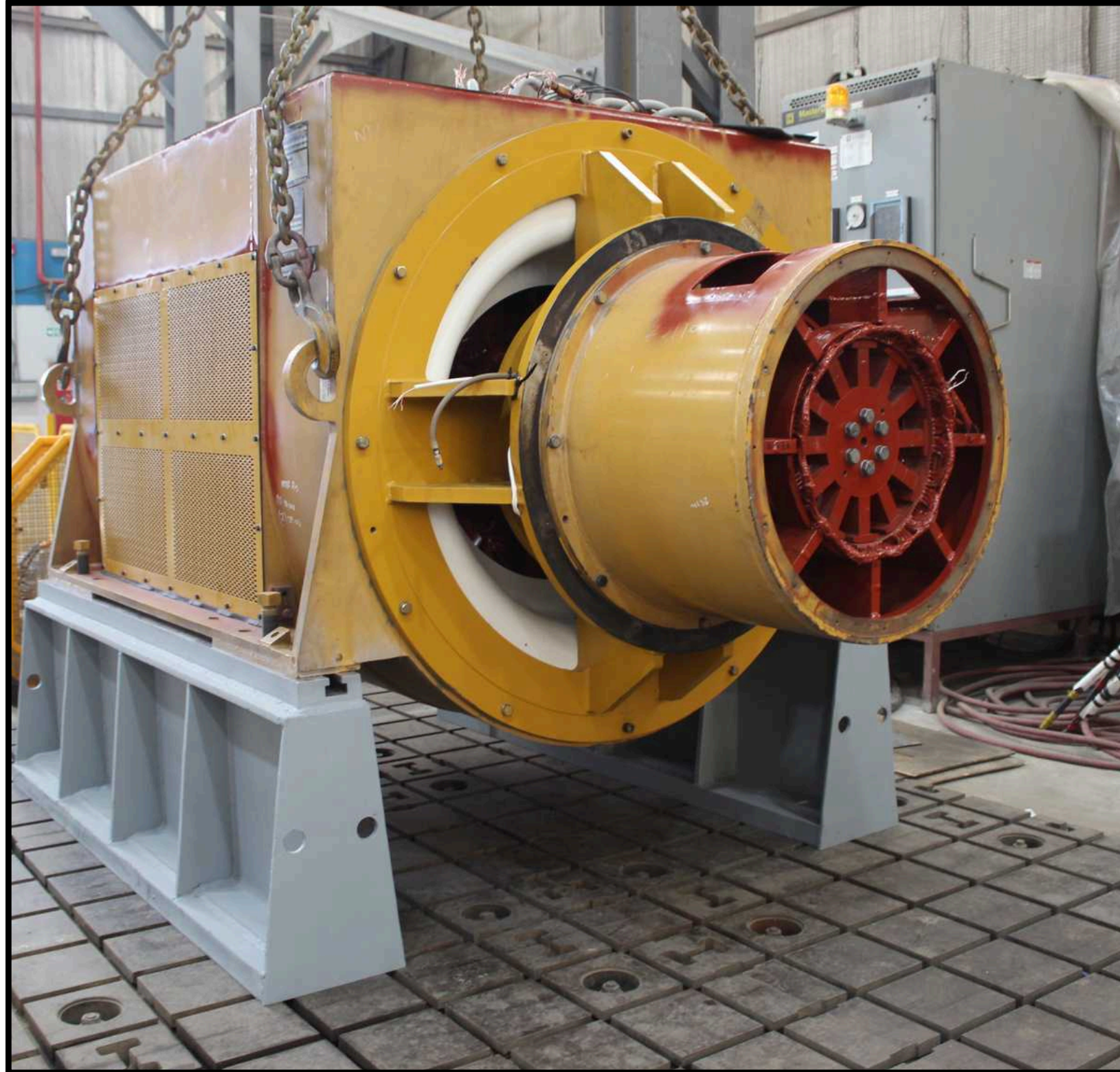
Generator Saection
