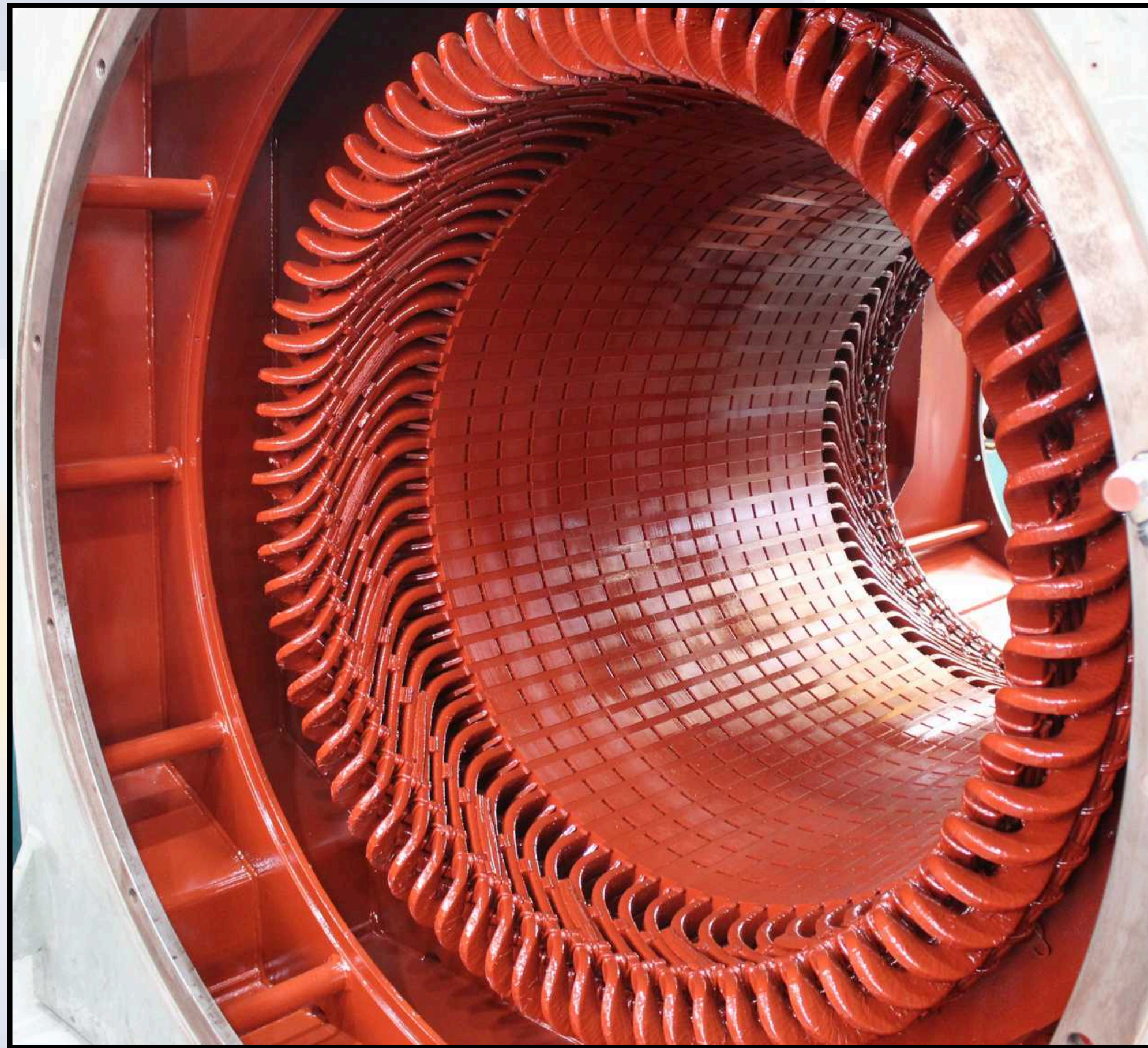
Rewinding Section
